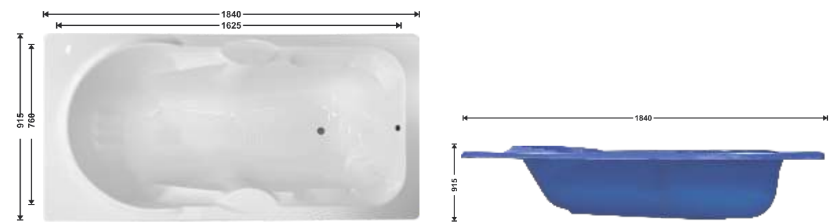
003- 6"x3" Length : 1840mm Breodths : 915mm Depth : 410mm Waste Hole Distance From Wall : 350mm
