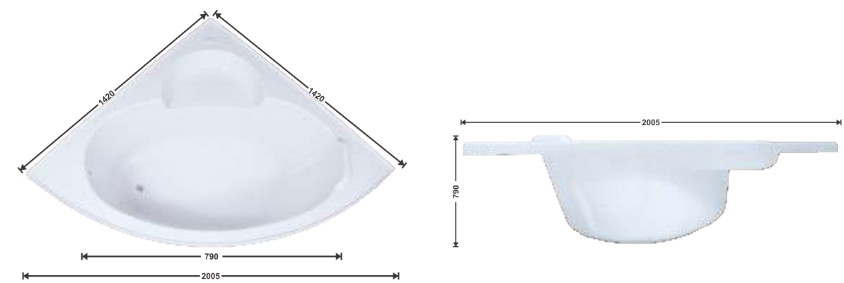
002- 56"x56" Length : 1420mm Breodths : 1420mm Depth : 405mm Waste Hole Distance From Wall : 455mm
