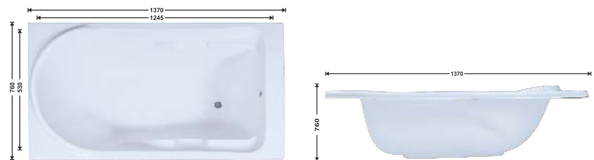
006- 4.5"x2.5" Length : 1370mm Breodths : 760mm Depth : 415mm Waste Hole Distance From Wall : 410mm
