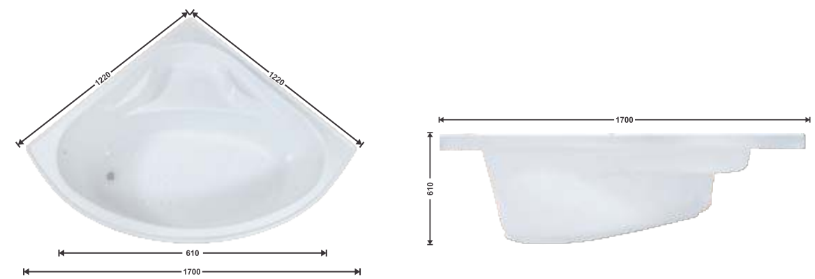
001- 48"x48" Length : 1220mm Breodths : 1220mm Depth : 410mm Waste Hole Distance From Wall : 455mm
