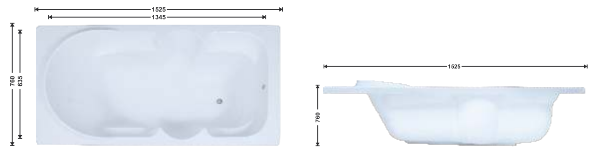
005- 5.5"x2.5" Length : 1525mm Breodths : 760mm Depth : 405mm Waste Hole Distance From Wall : 350mm
